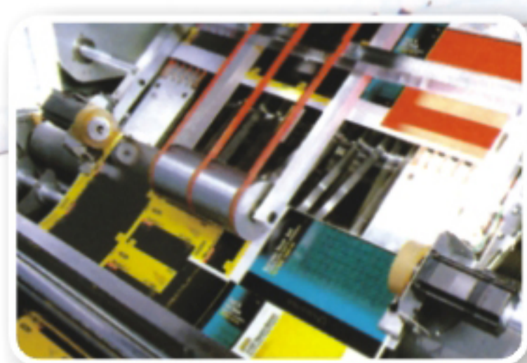
PAPER ALIGNING SYSTEM 紙張感測補償對位系統
