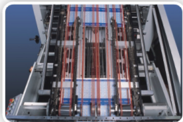
DYNAM ALIGNING MECHANISM 動態規位機構
