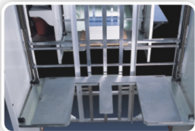
LOW FRAME E STYLE PALLET LOADER 低台側移式E型托紙架
